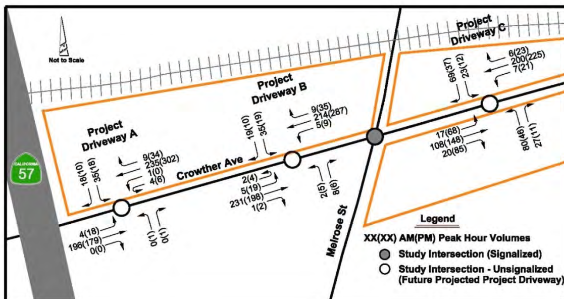
Figure 2-6. Existing 2016 with Project - Project Driveway Volumes
