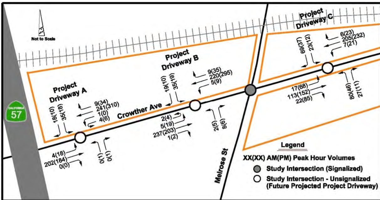
Figure 3-3. Opening Day 2018 with Project - Project Driveway Volumes
