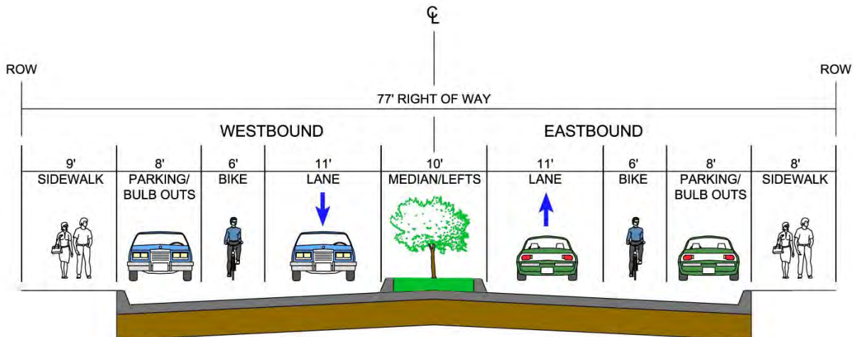
Figure 1-B. Crowther Avenue as a Two-Lane Facility
