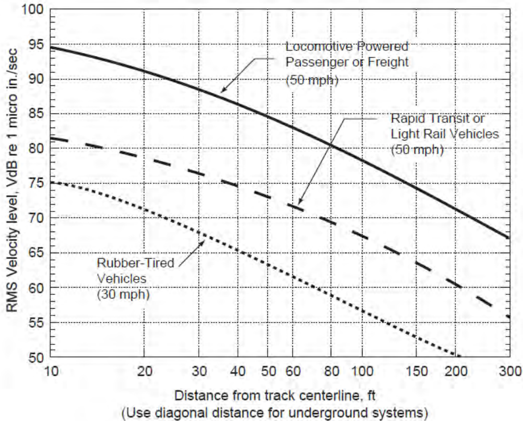
FIGURE 4 GENERALIZE GROUND SURFACE VIBRATION CURVES
