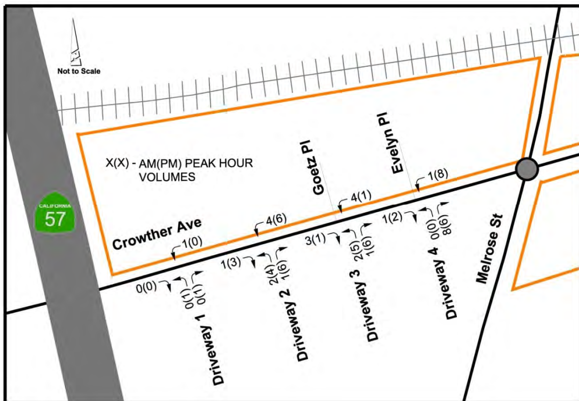
Figure 2-5b. Existing 2016 South Driveway Volumes
