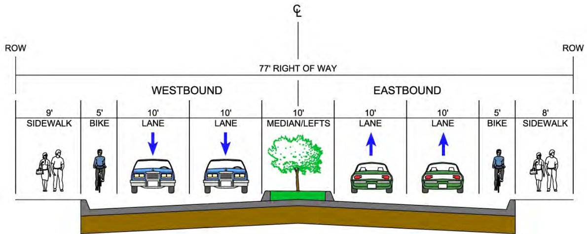
Figure 1-A. Crowther Avenue as a Four-Lane Facility
