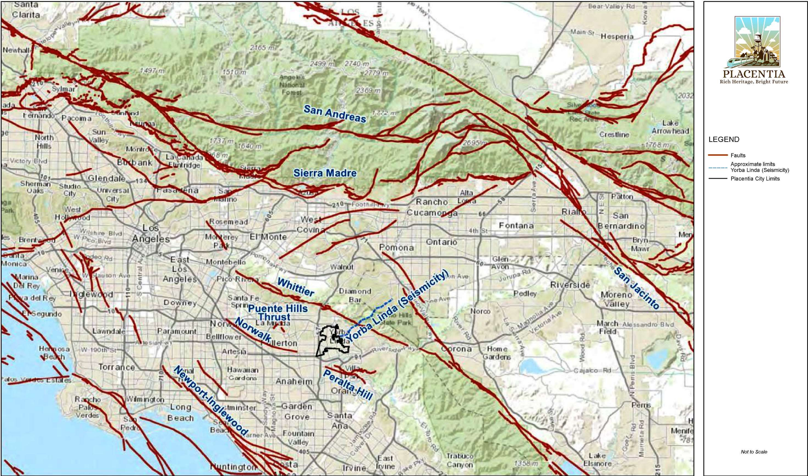
Exhibit 7-1. Regional Faults
